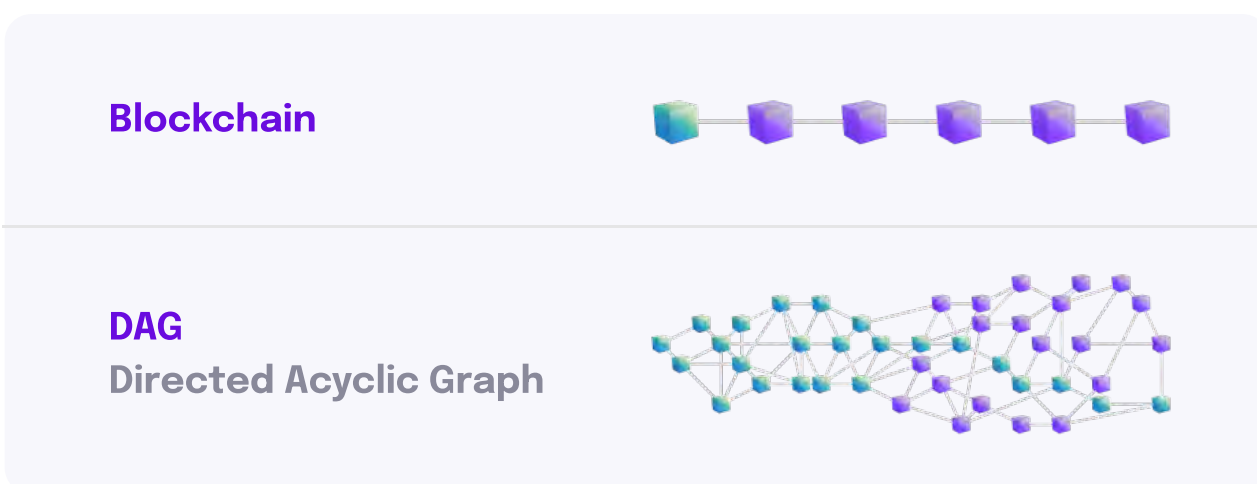
Figure 5.1 Blockchain structure vs. Directed Acyclic Graph structure
